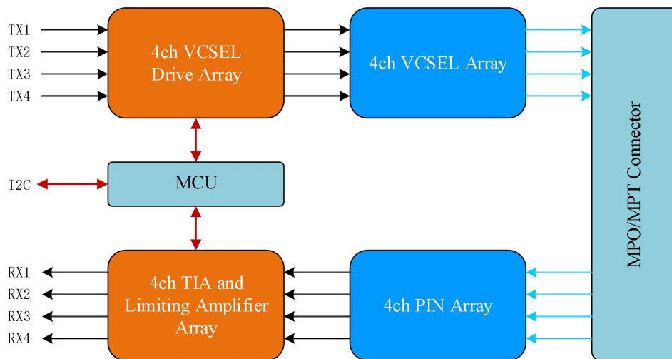
Figure1: Block Diagram
