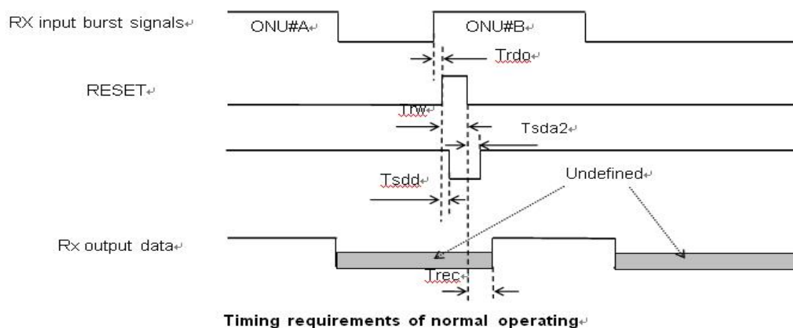
Figure 3 Timing Parameter Definitions in Burst Mode Sequence
